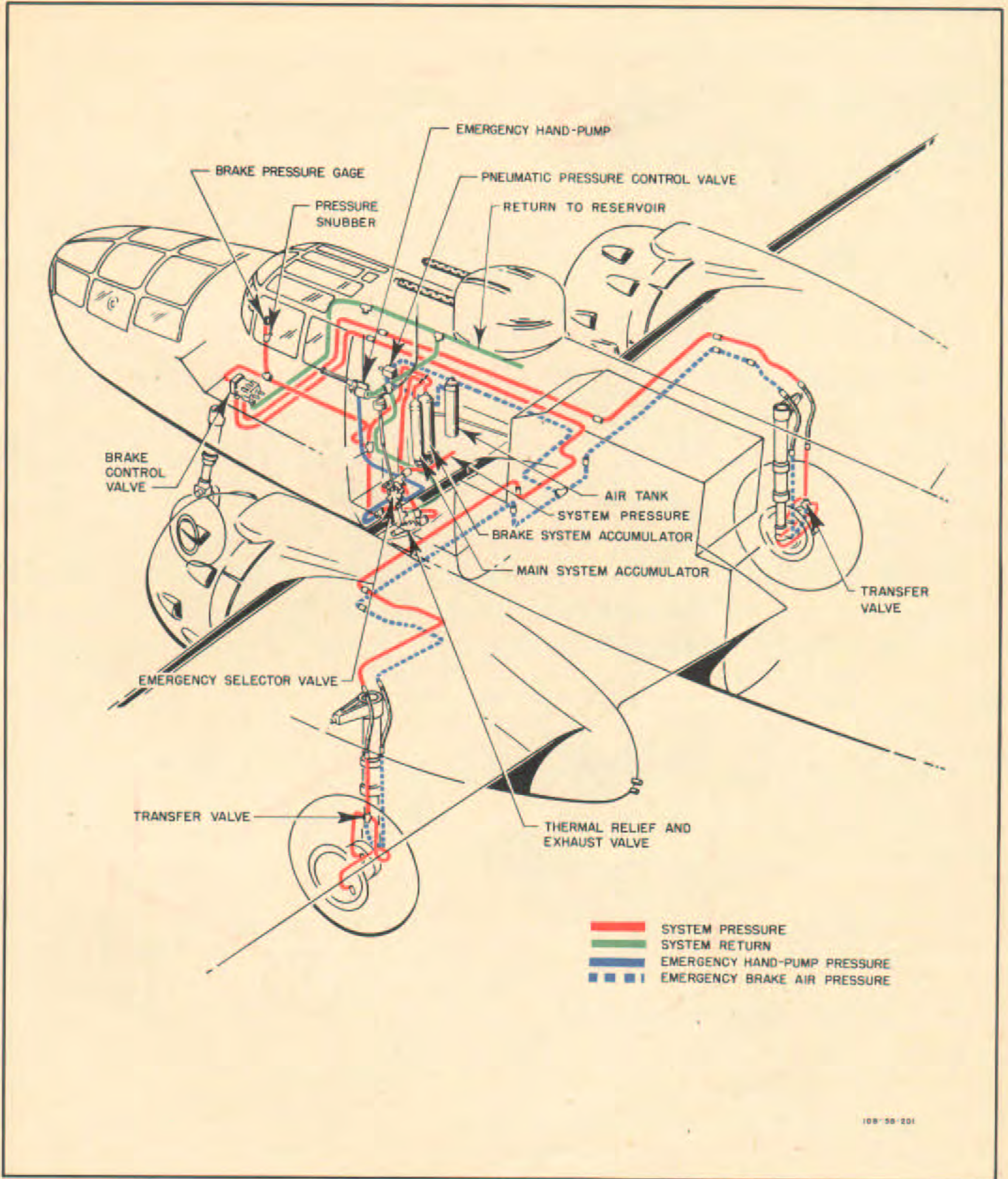
Figure 10—Hydraulic Brake and Emergency Air Brake Systems
