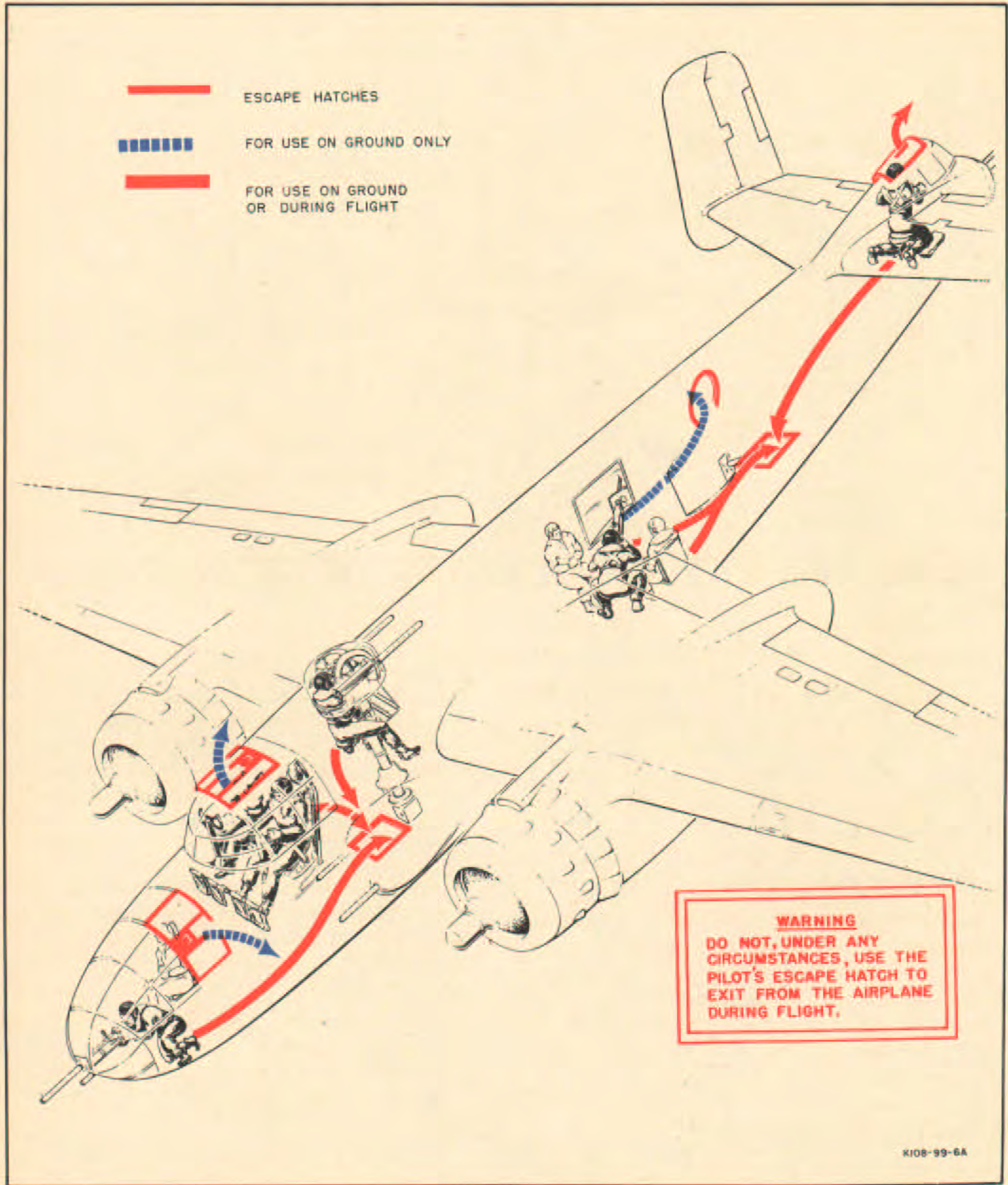
Figure 31—Emergency Exits
