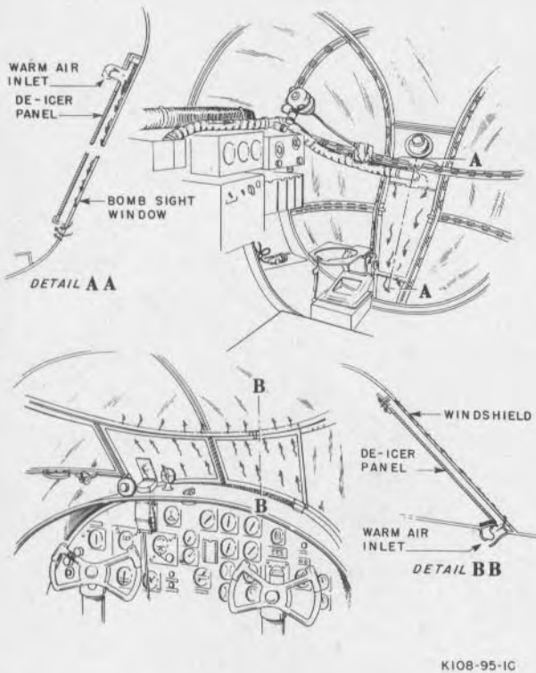
Figure 17—Defroster Panels
