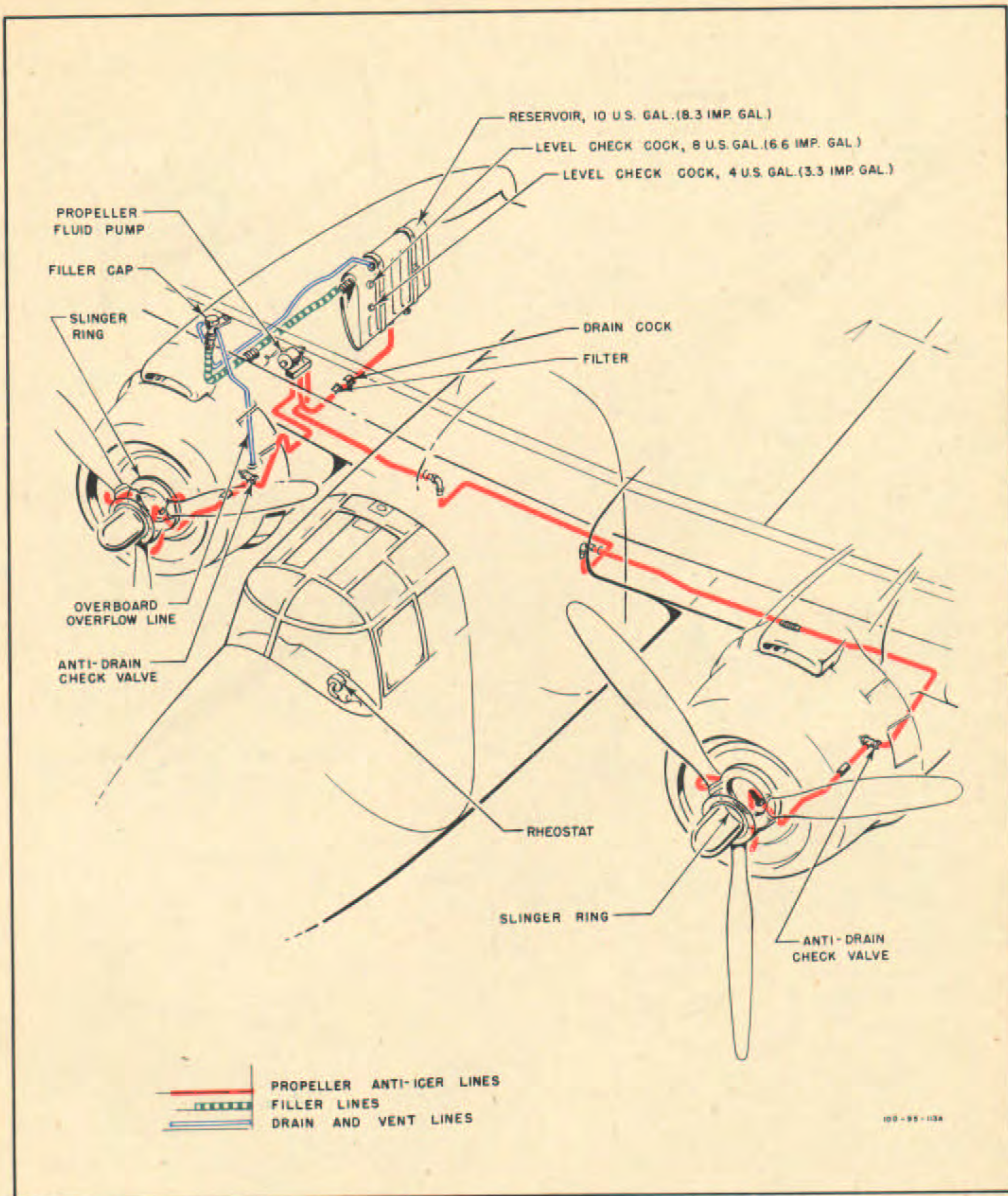
Figure 45—Propeller Anti-icer System
