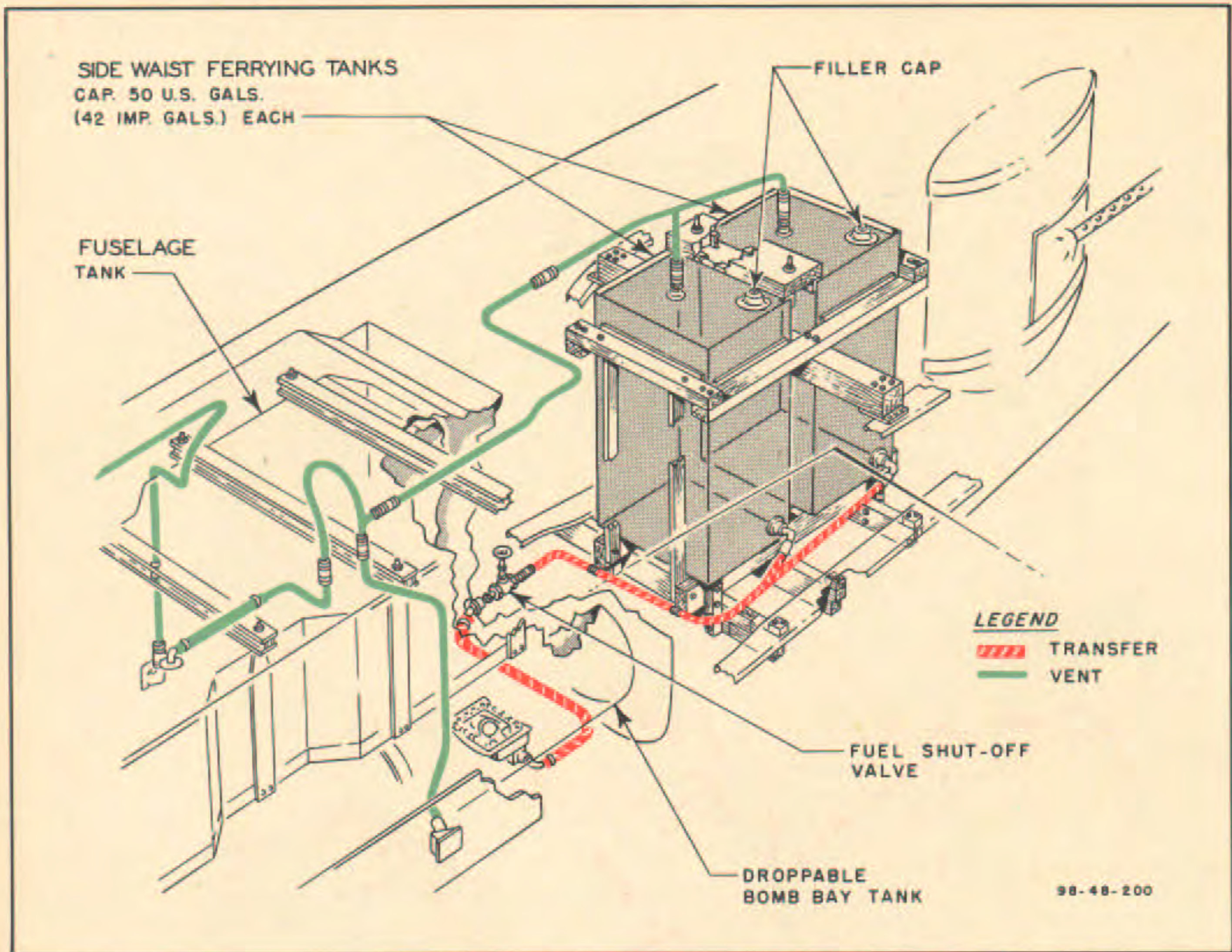
Figure 13- SIDE WAIST FERRYING TANKS
