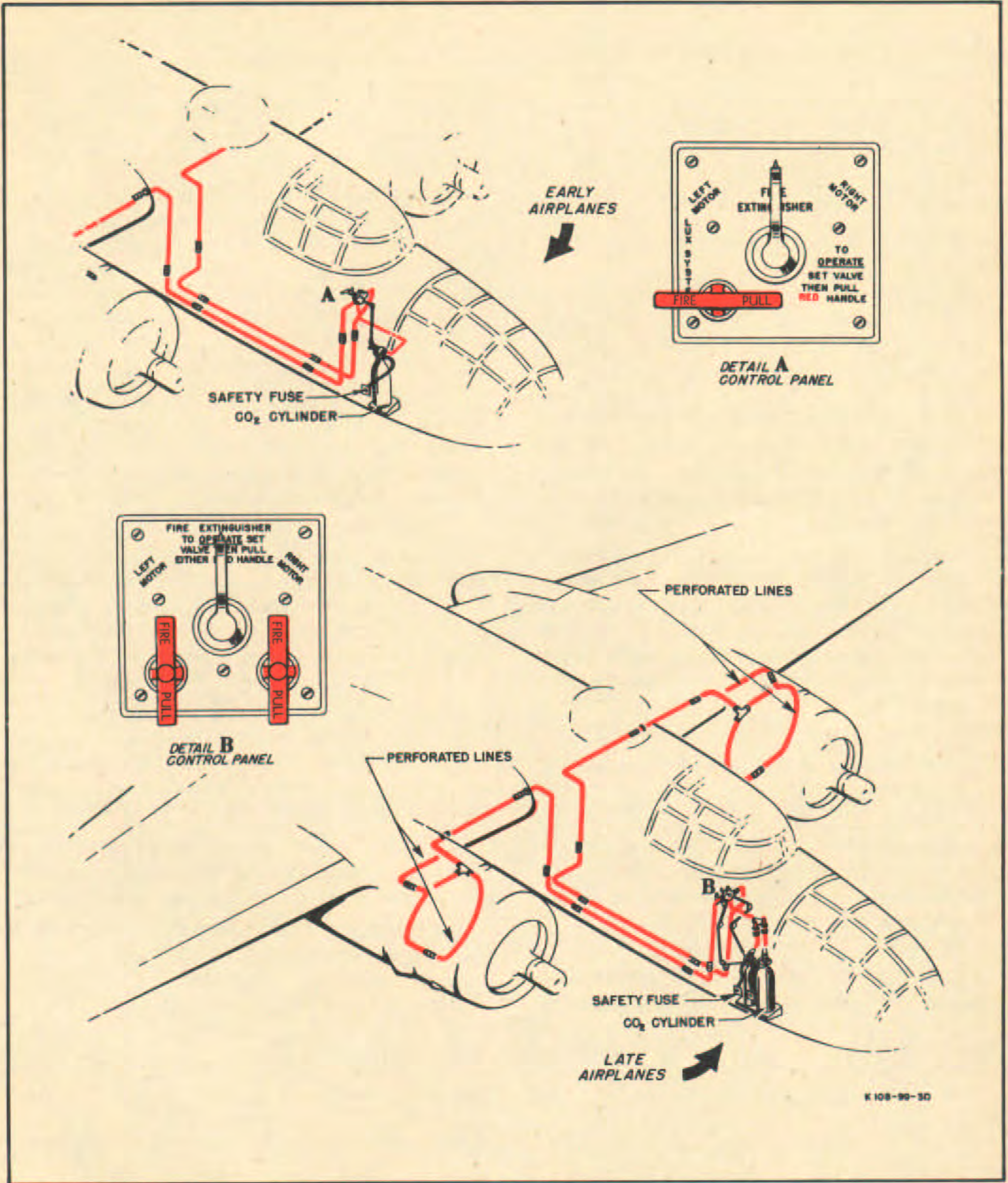
Figure 35—Engine Fire Extinguisher Systems
