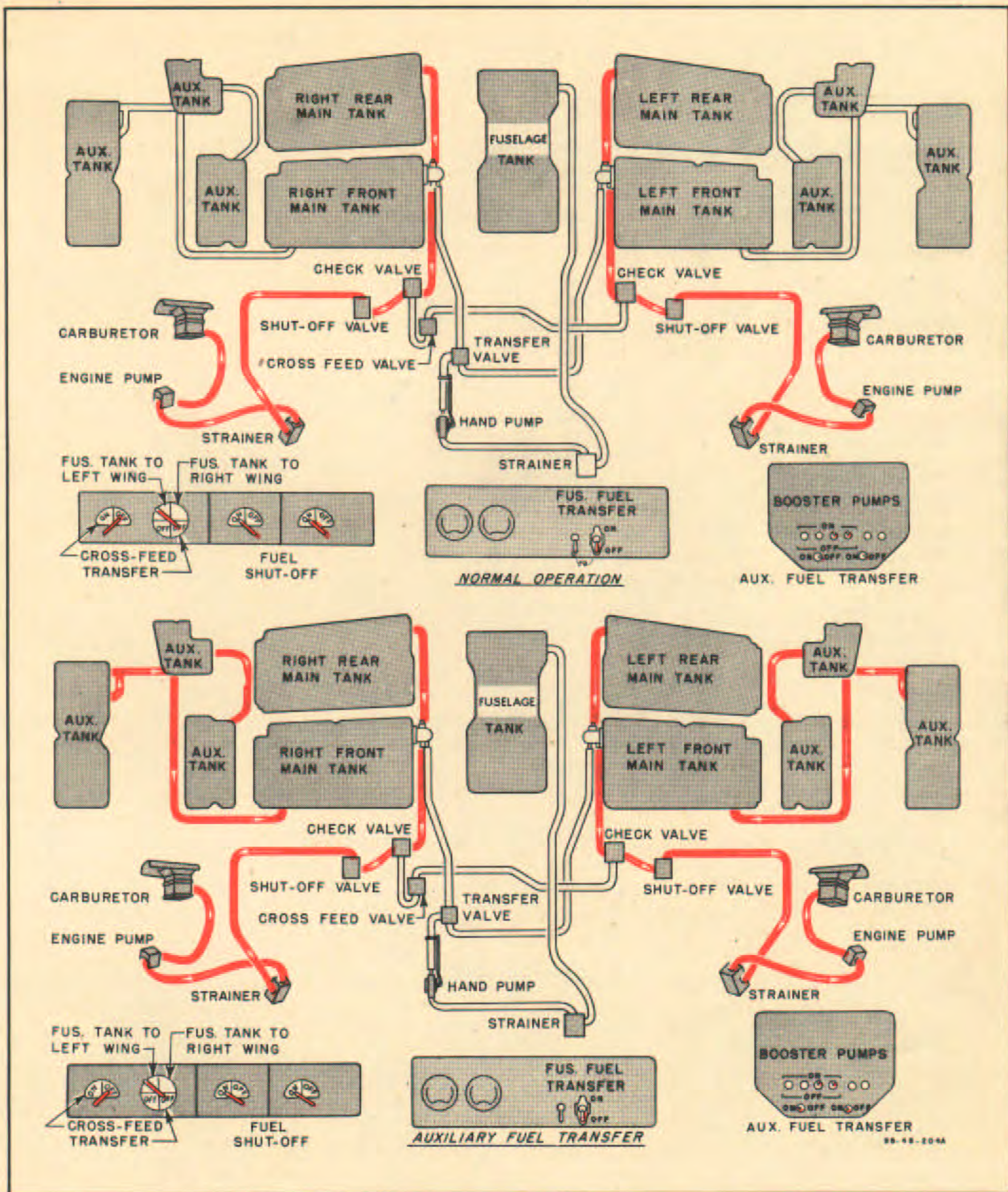
Figure 22—Fuel System Management—Normal Operation Auxiliary Transfer
