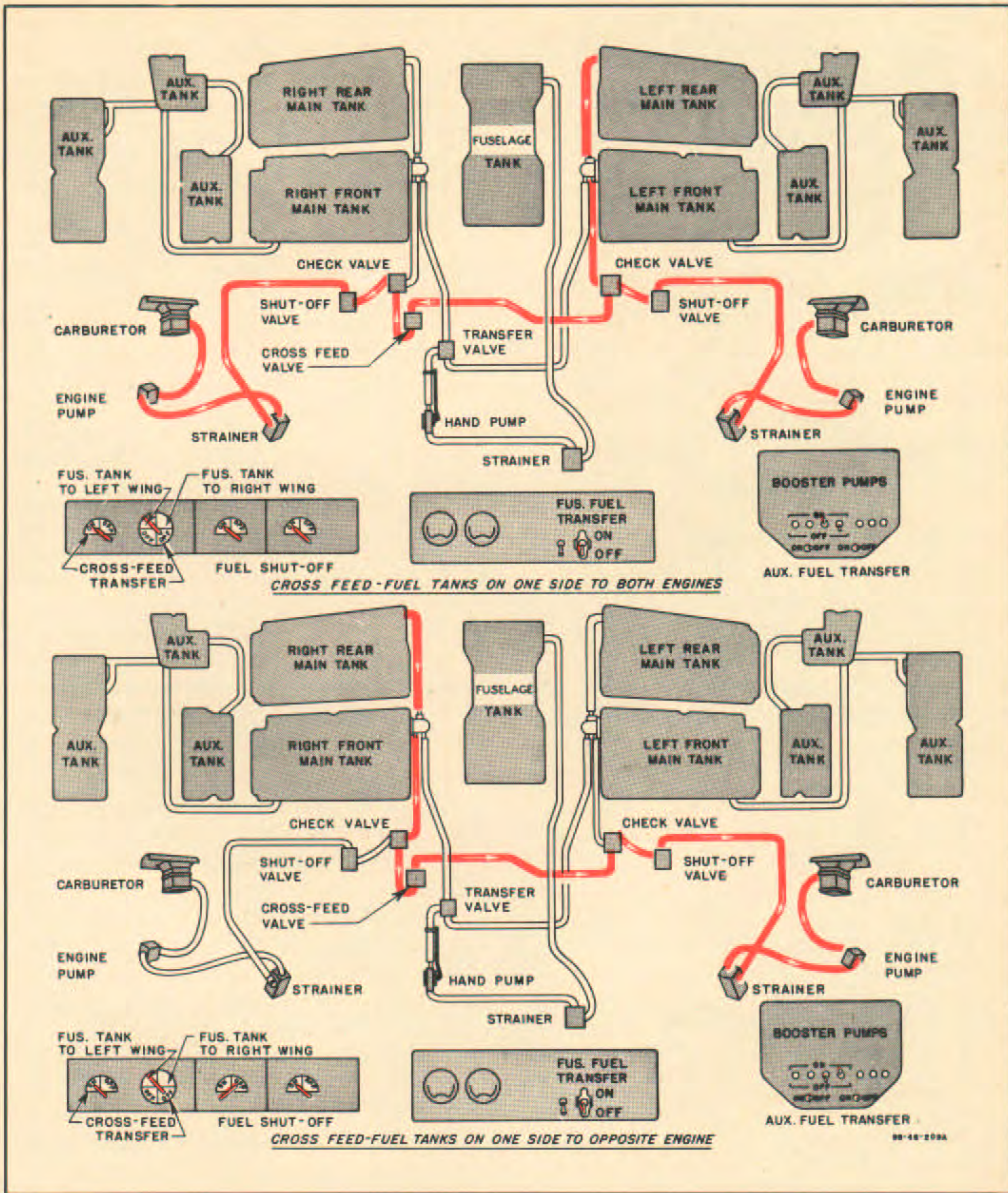
Figure 24—Fuel System Management—Cross Feed
