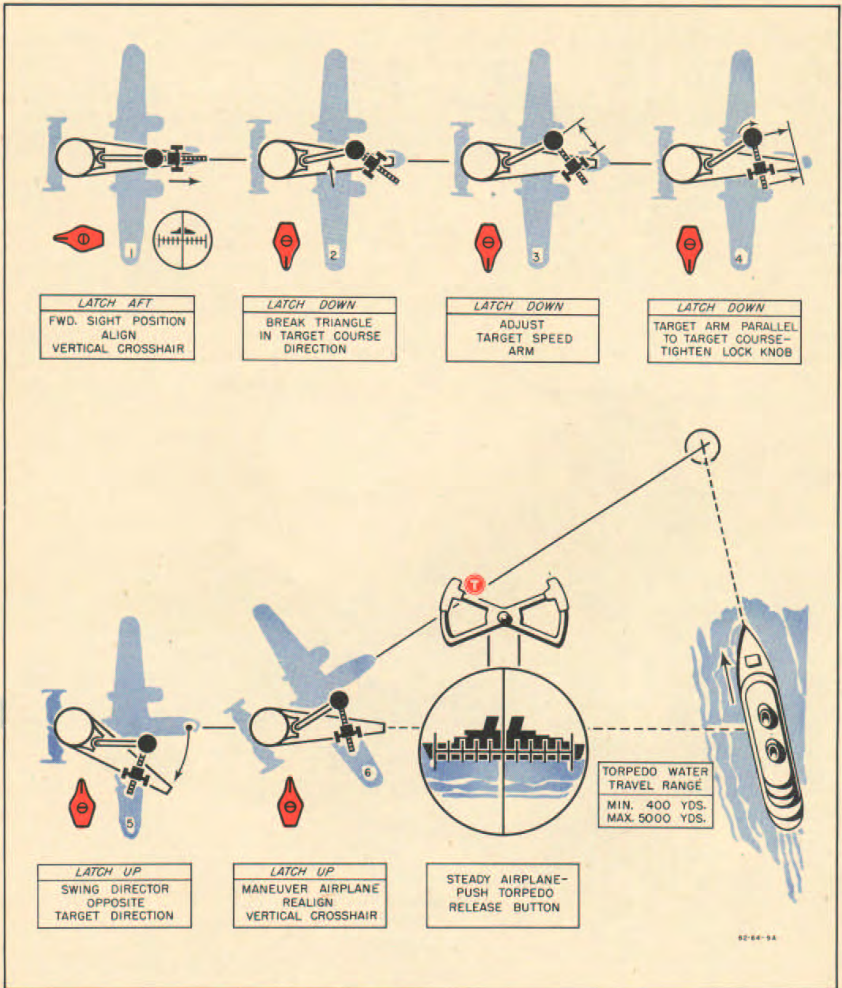
Figure 39—Operation of Torpedo Director
