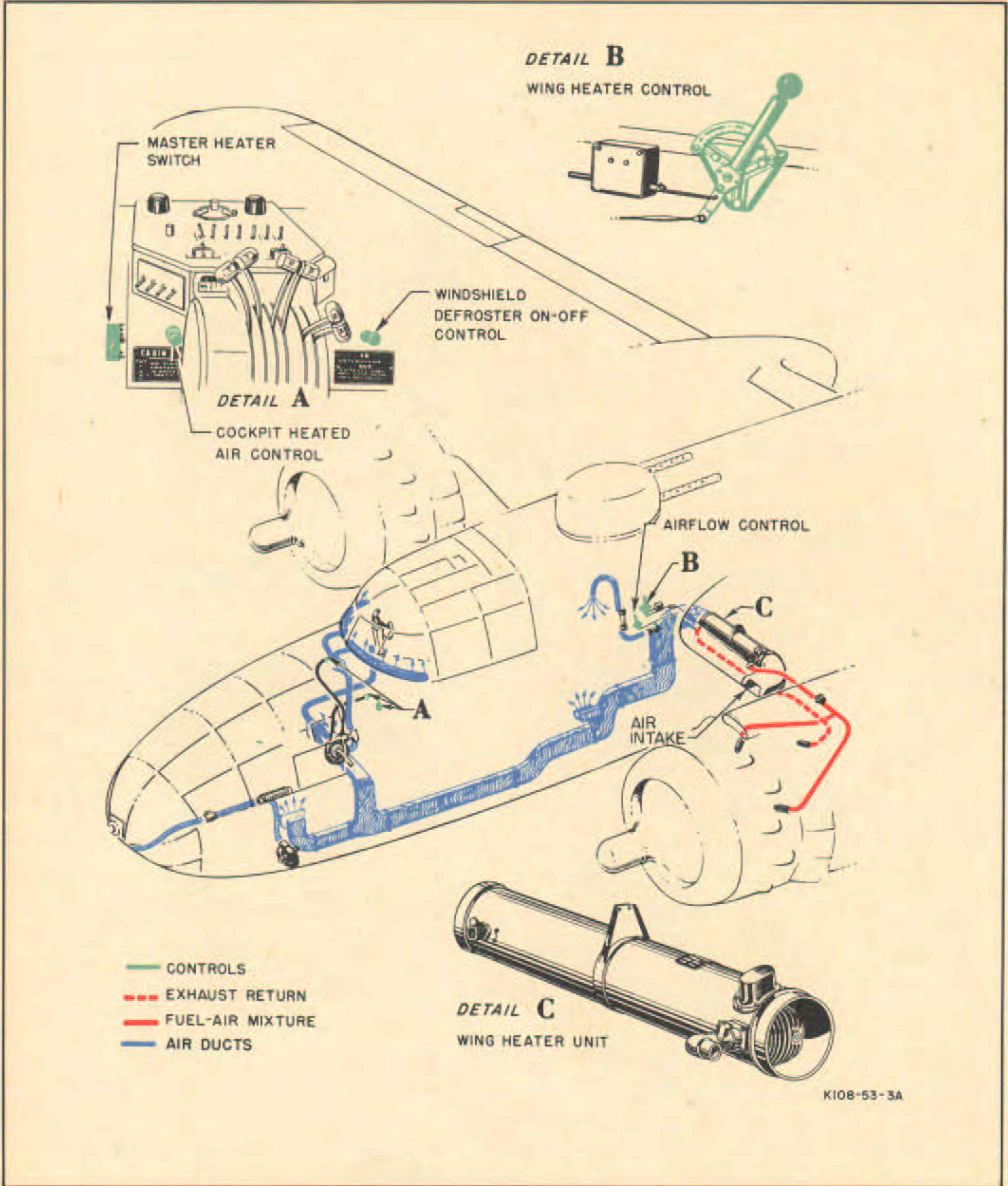
Figure 15—Heating and Ventilating System—Forward
