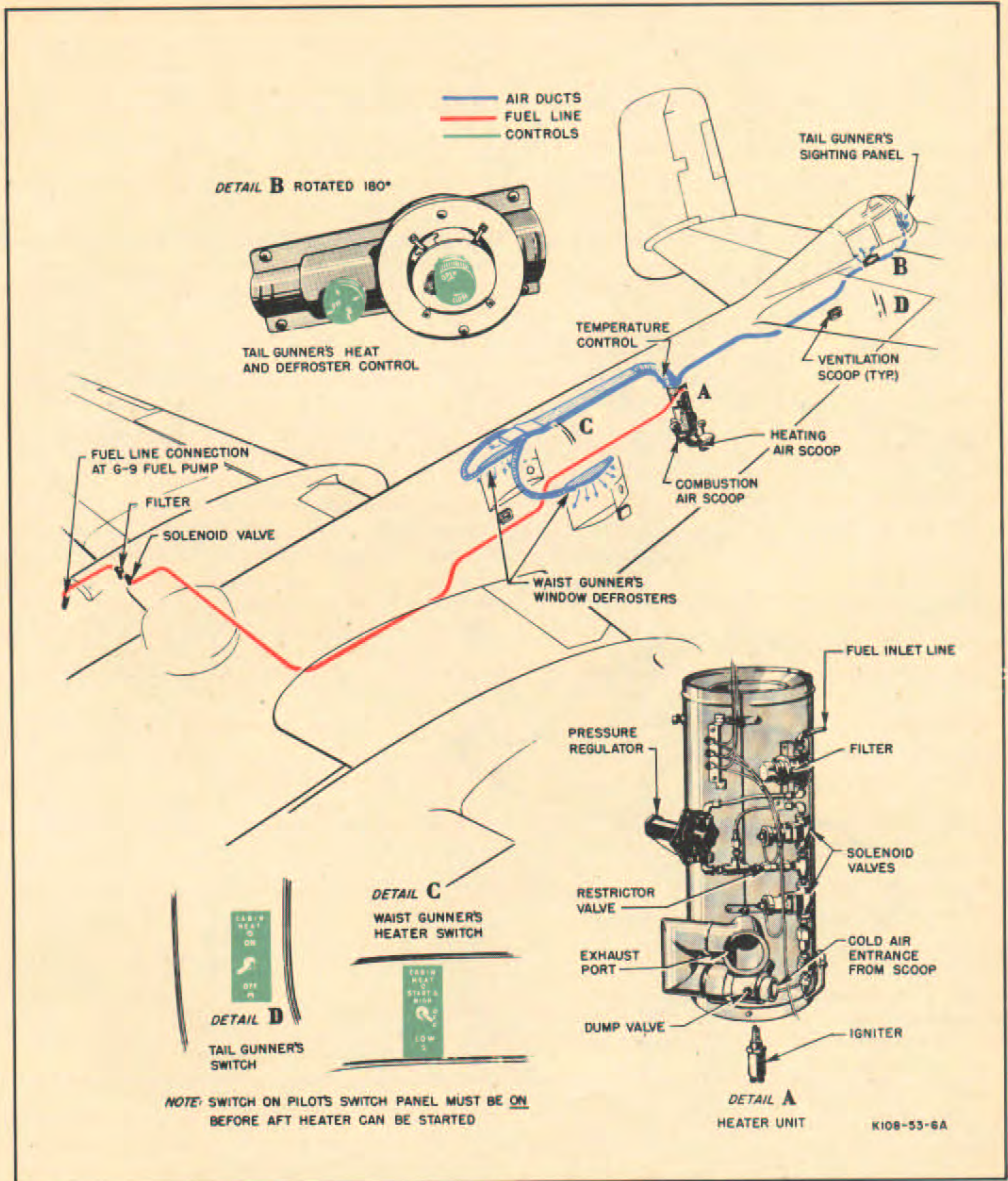
Figure 16—Heating and Ventilating System—Rear
