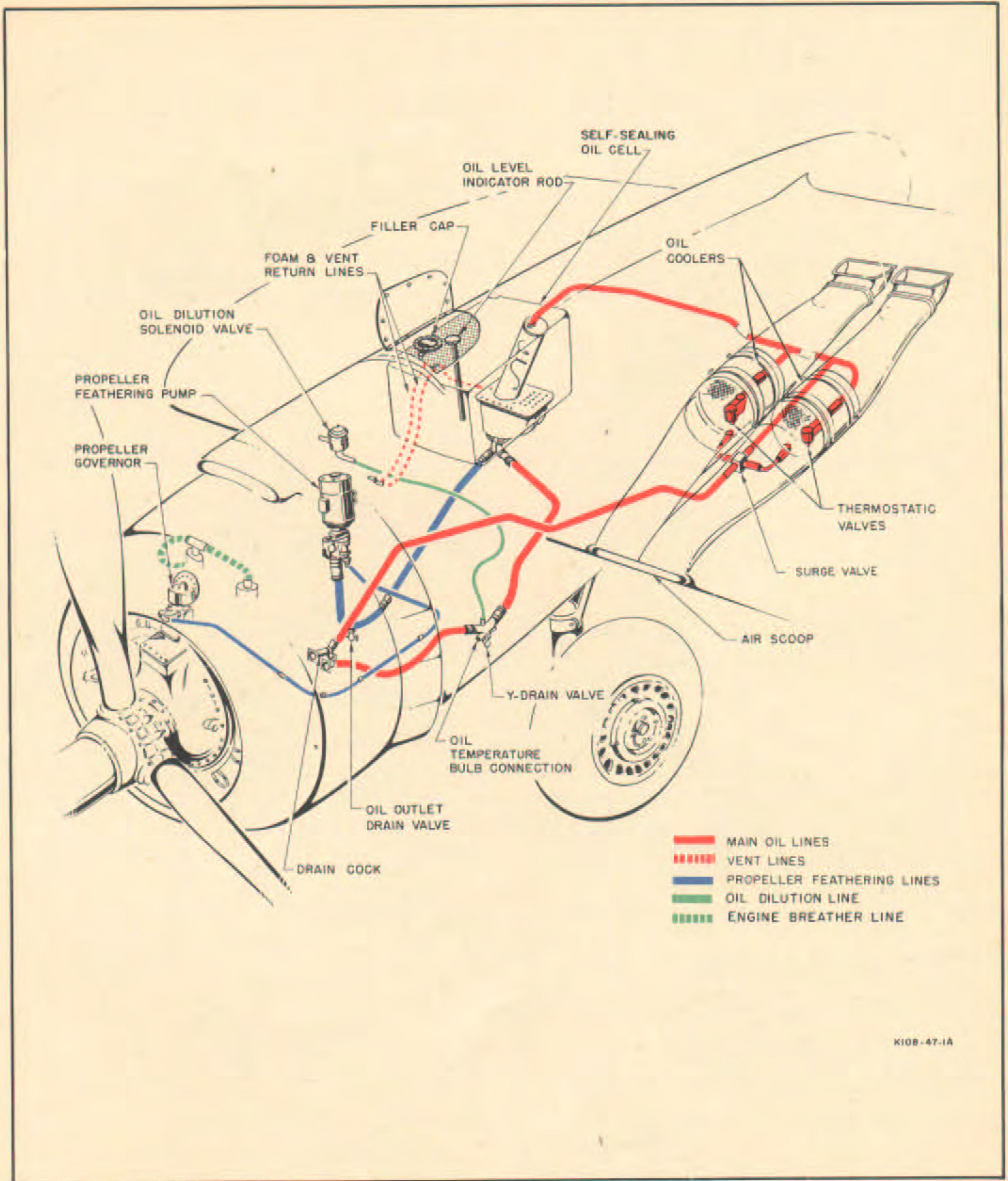
Figure 14—Oil System
