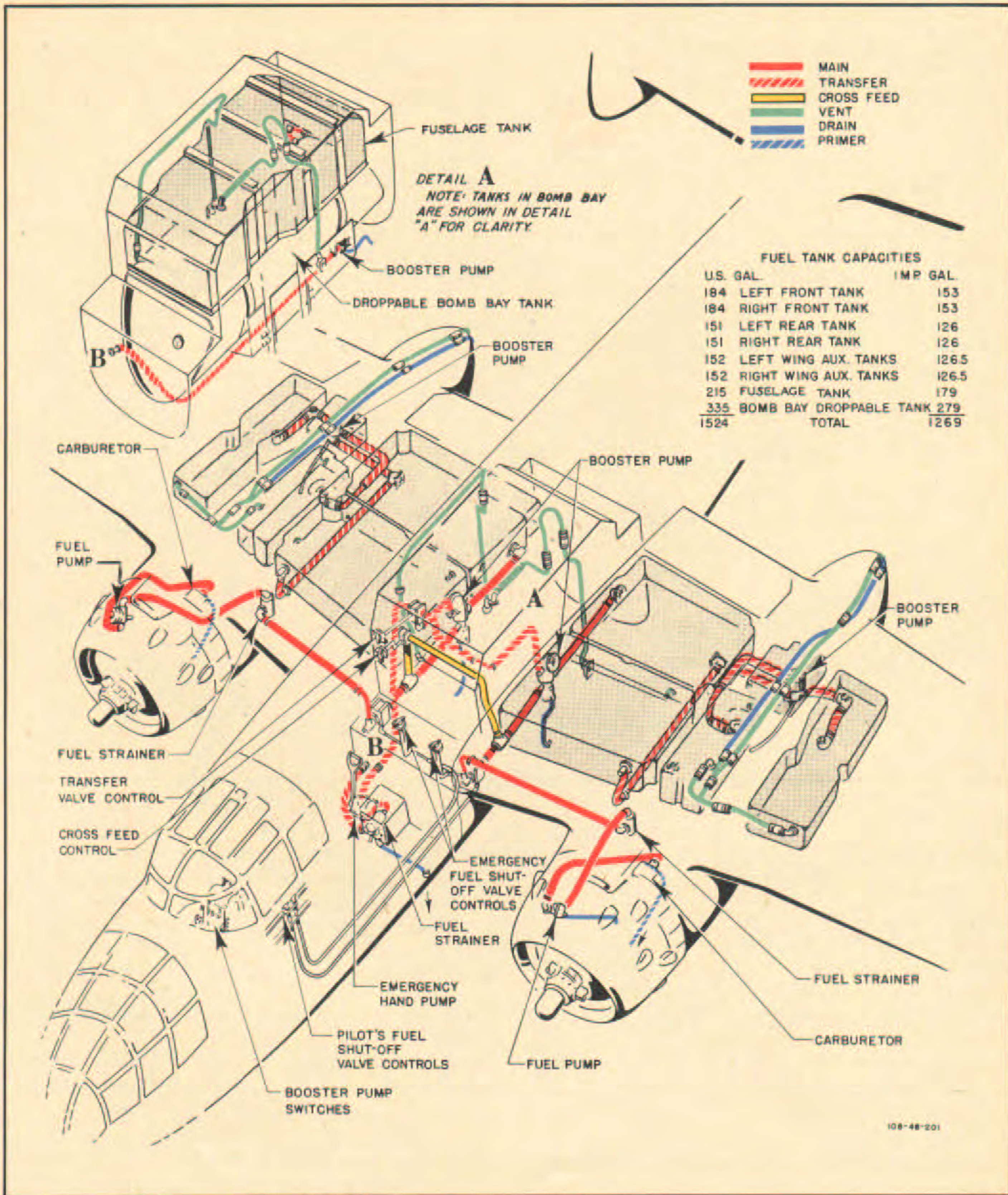
Figure 12—Fuel System
