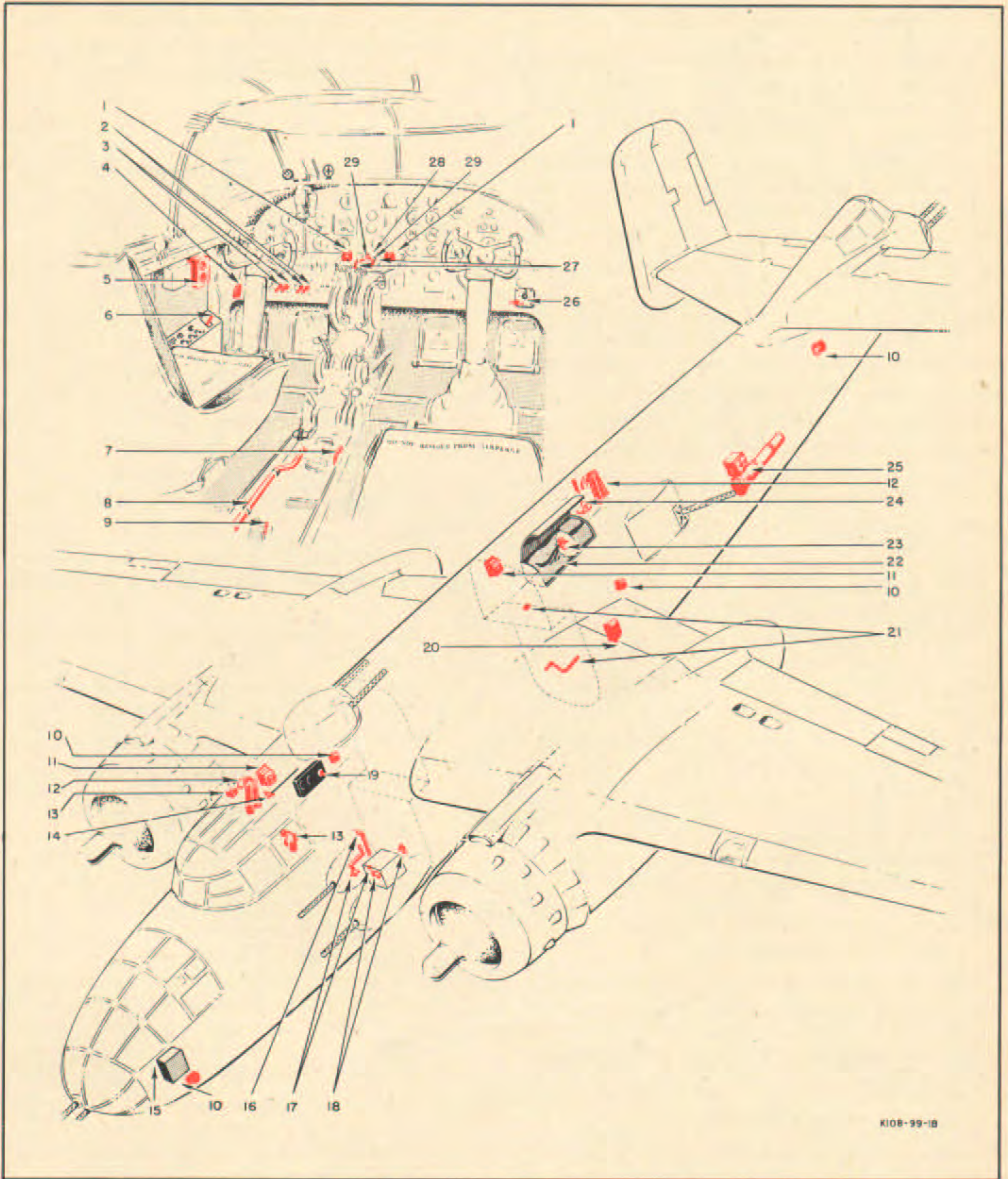
Figure 34—Emergency Equipment
