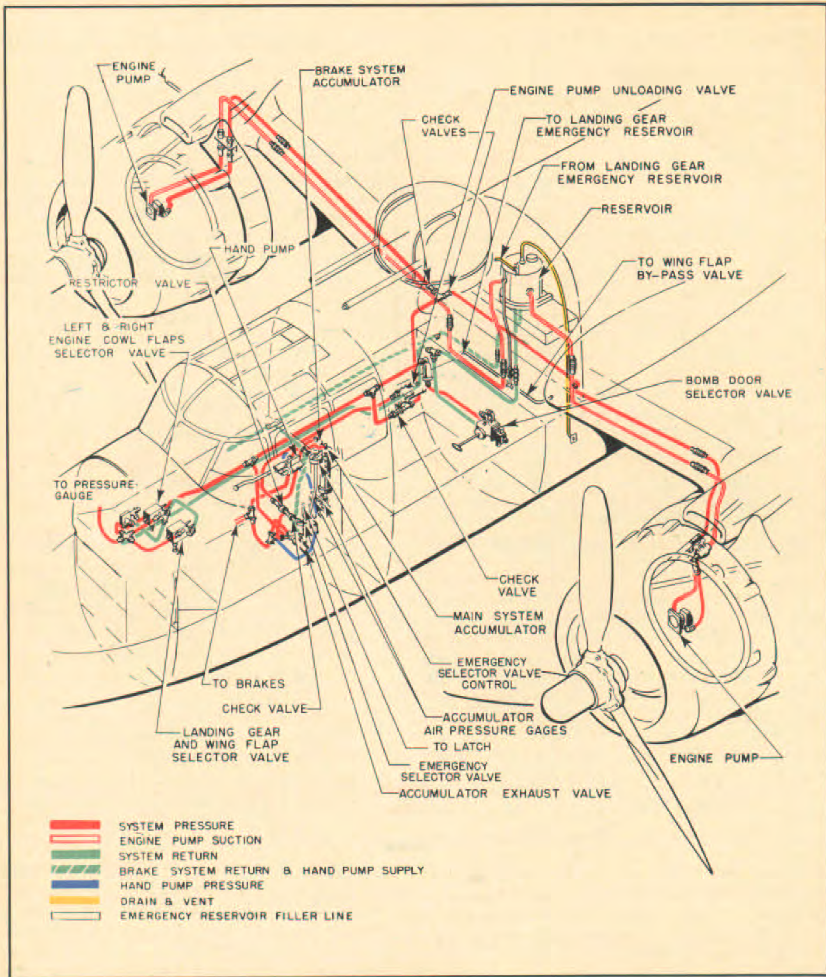
Figure 7—Hydraulic Power System
