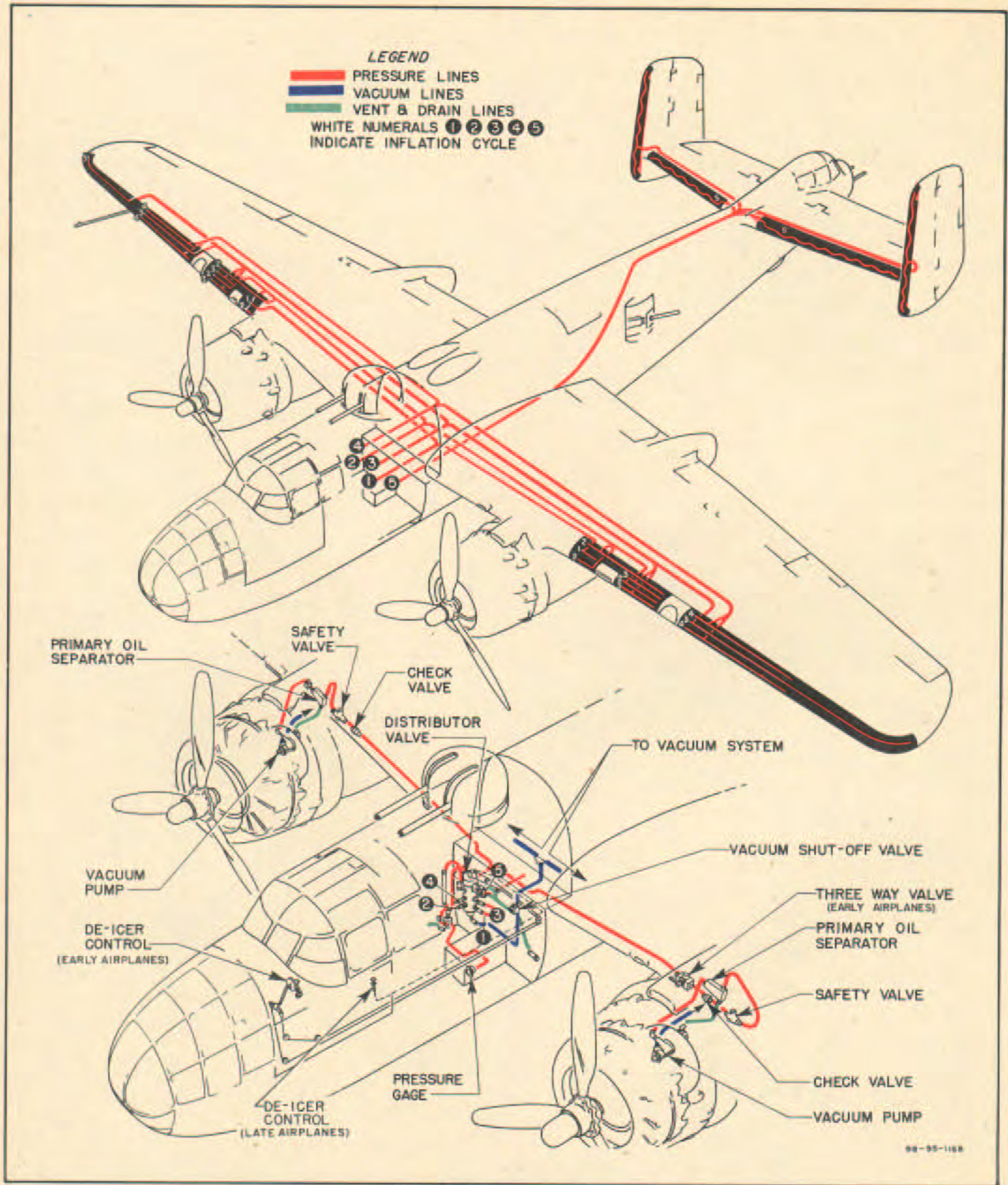
Figure 46—Surface De-icer System
