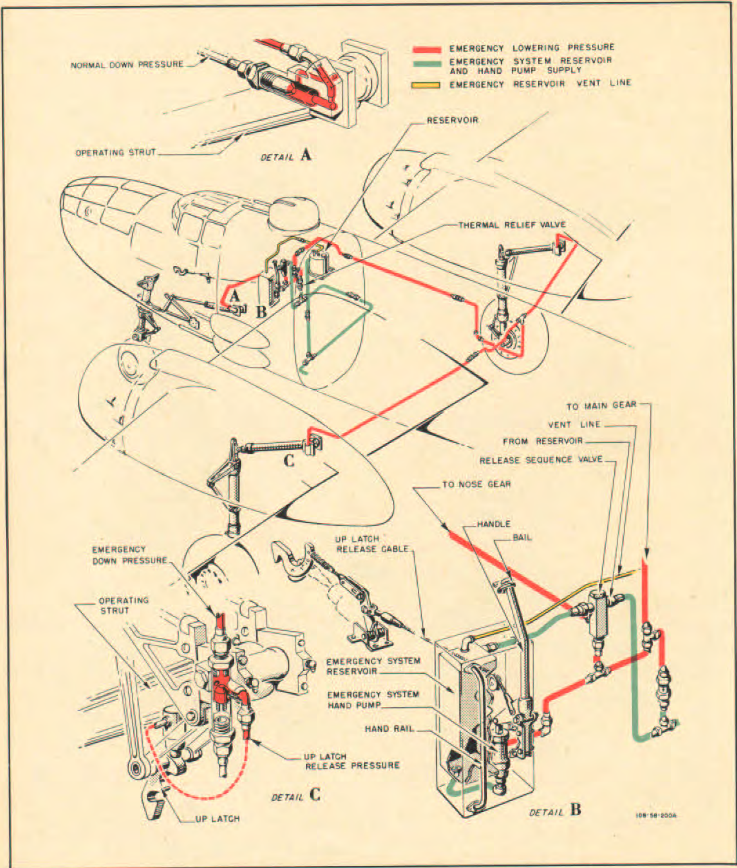
Figure 11—Landing Gear Hydraulic Emergency Lowering System
