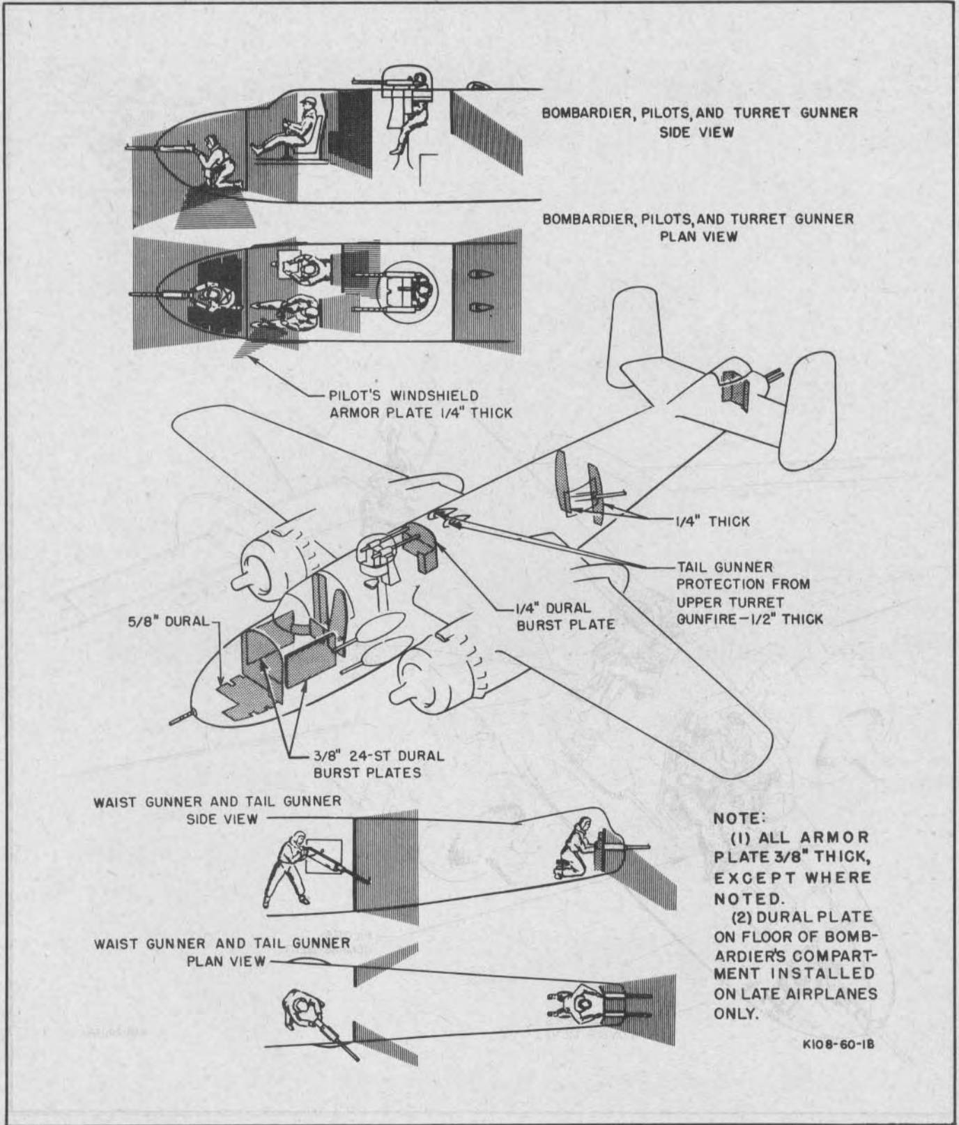
Figure 5—Armor Protection
