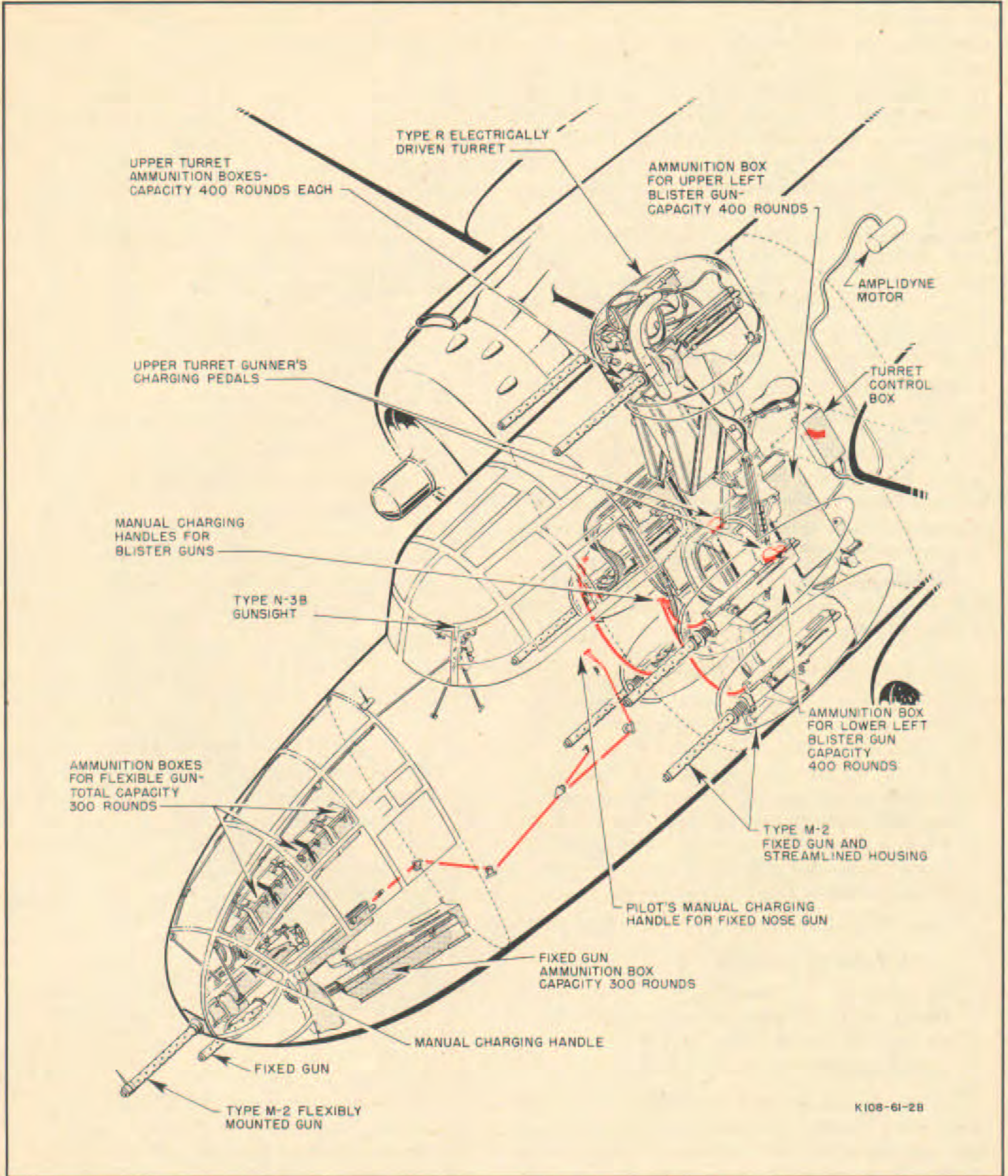
Figure 50—Gunnery Equipment—Front Section
