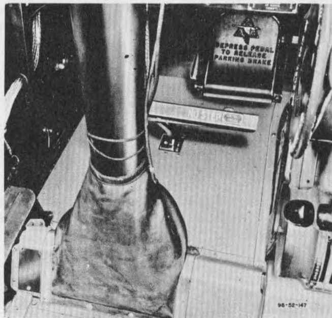
Figure 19—Surface Control Lock Handle
