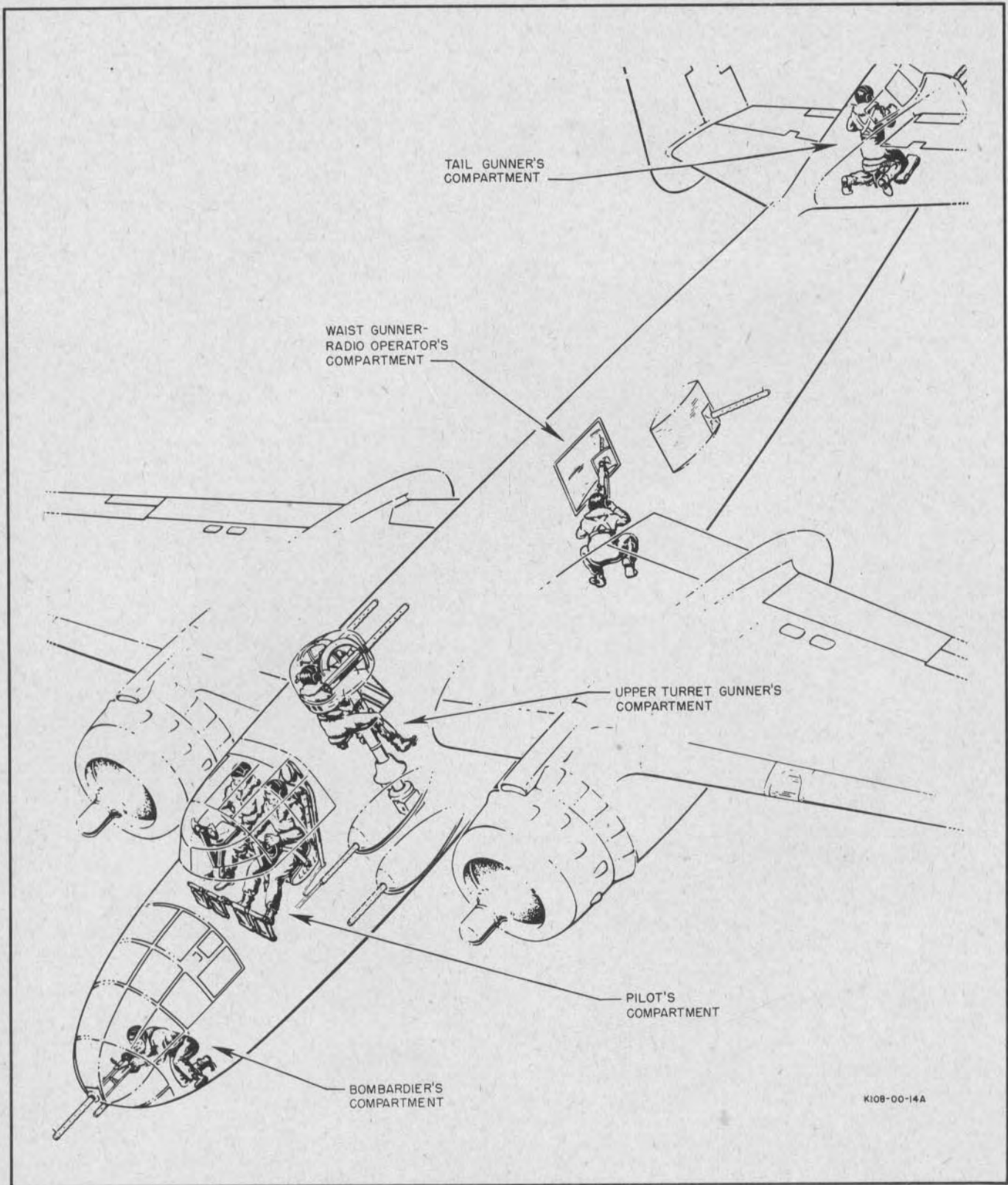
Figure 6—Fuselage Arrangement
