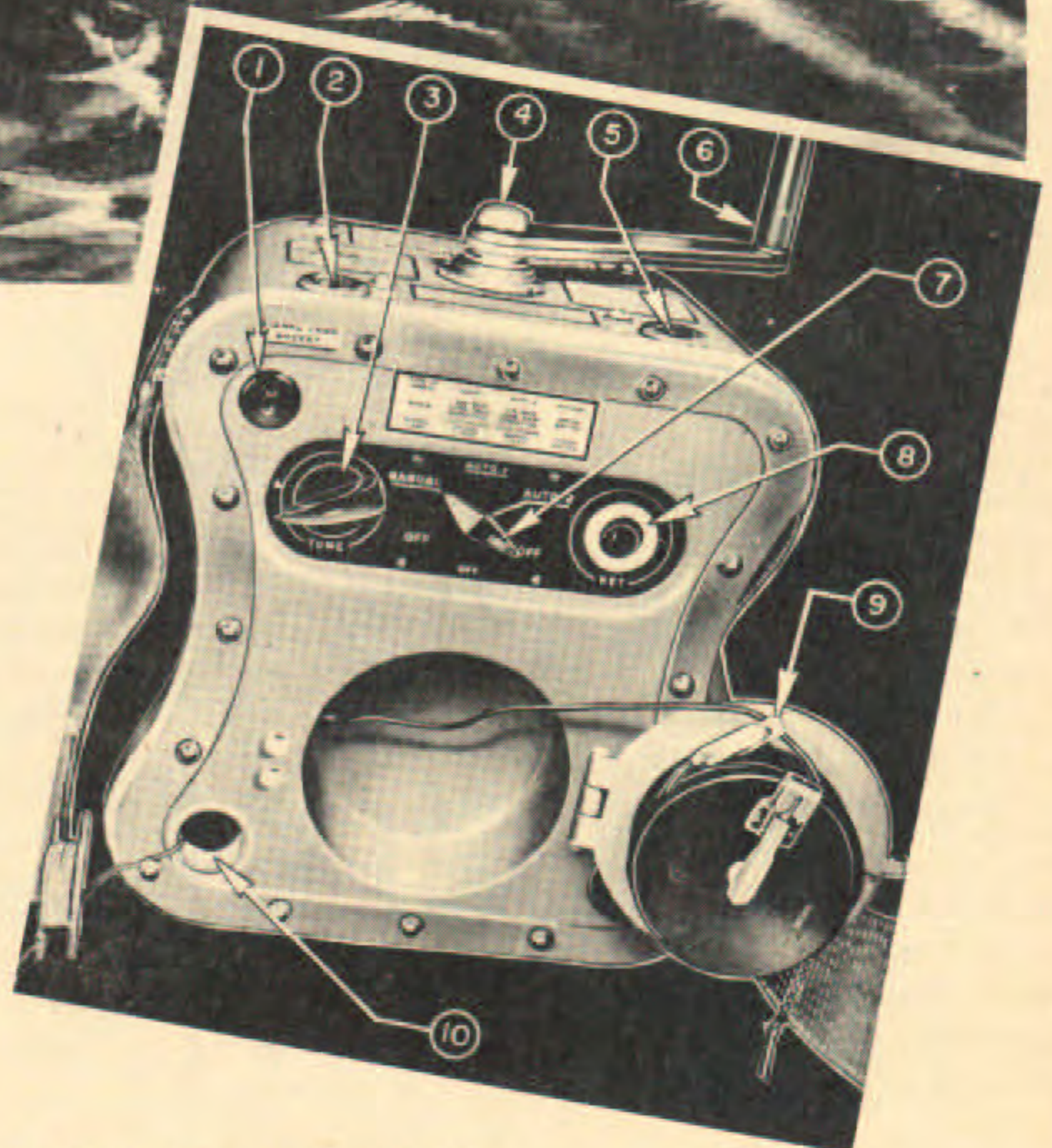
Figure 33—Dinghy Emergency Radio
