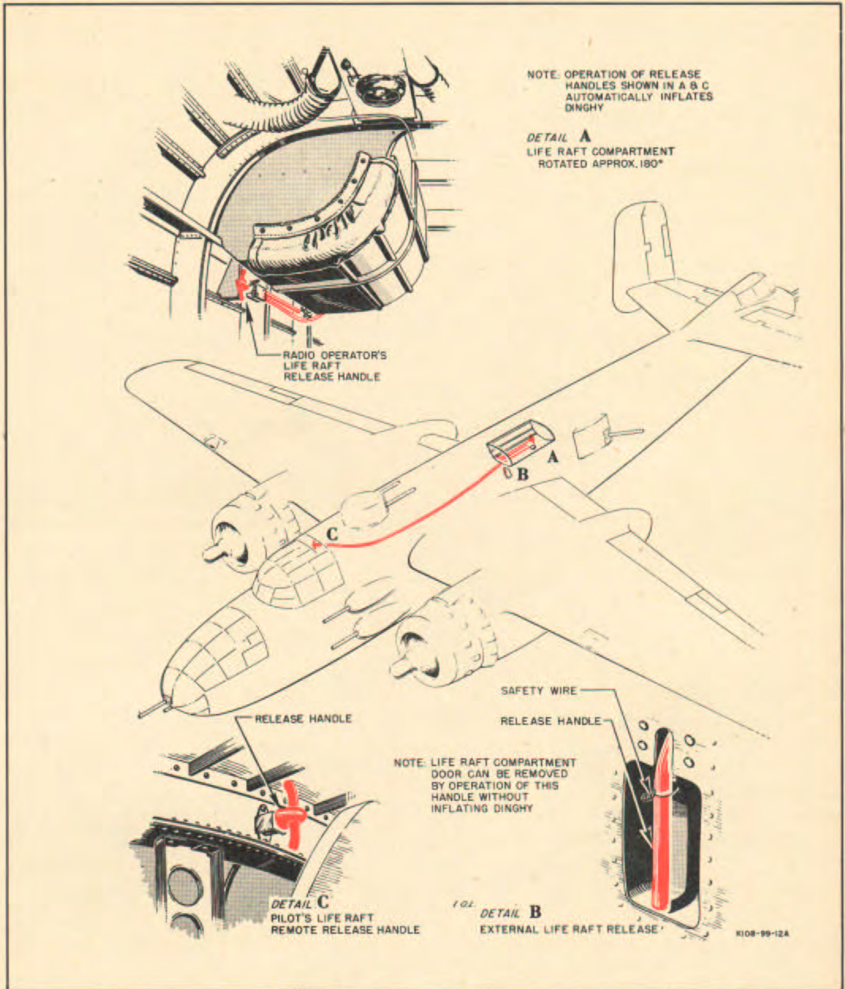
Figure 32—Life Raft Installation
