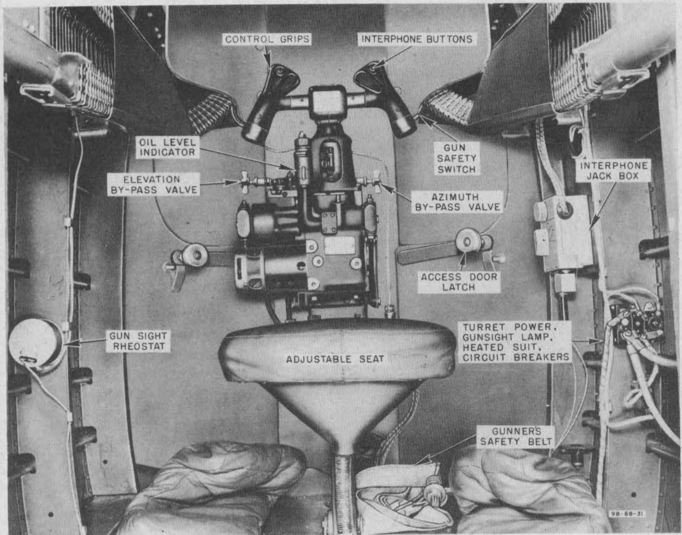
Figure 57—Tail Turret
