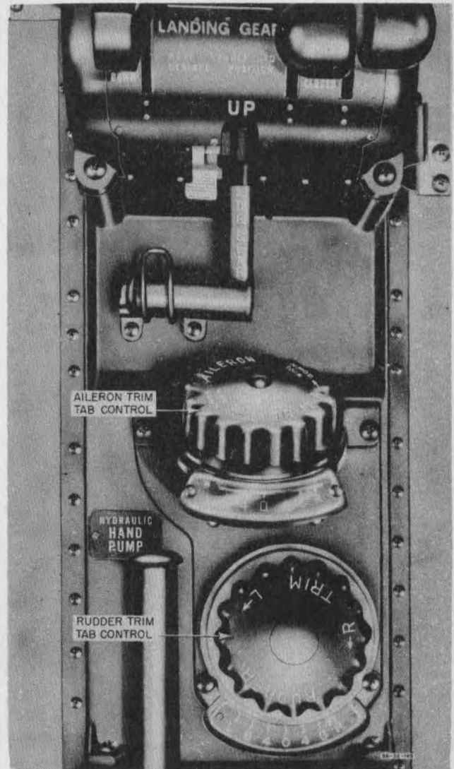
Figure 27—Aileron and Rudder Trim Tab Controls
