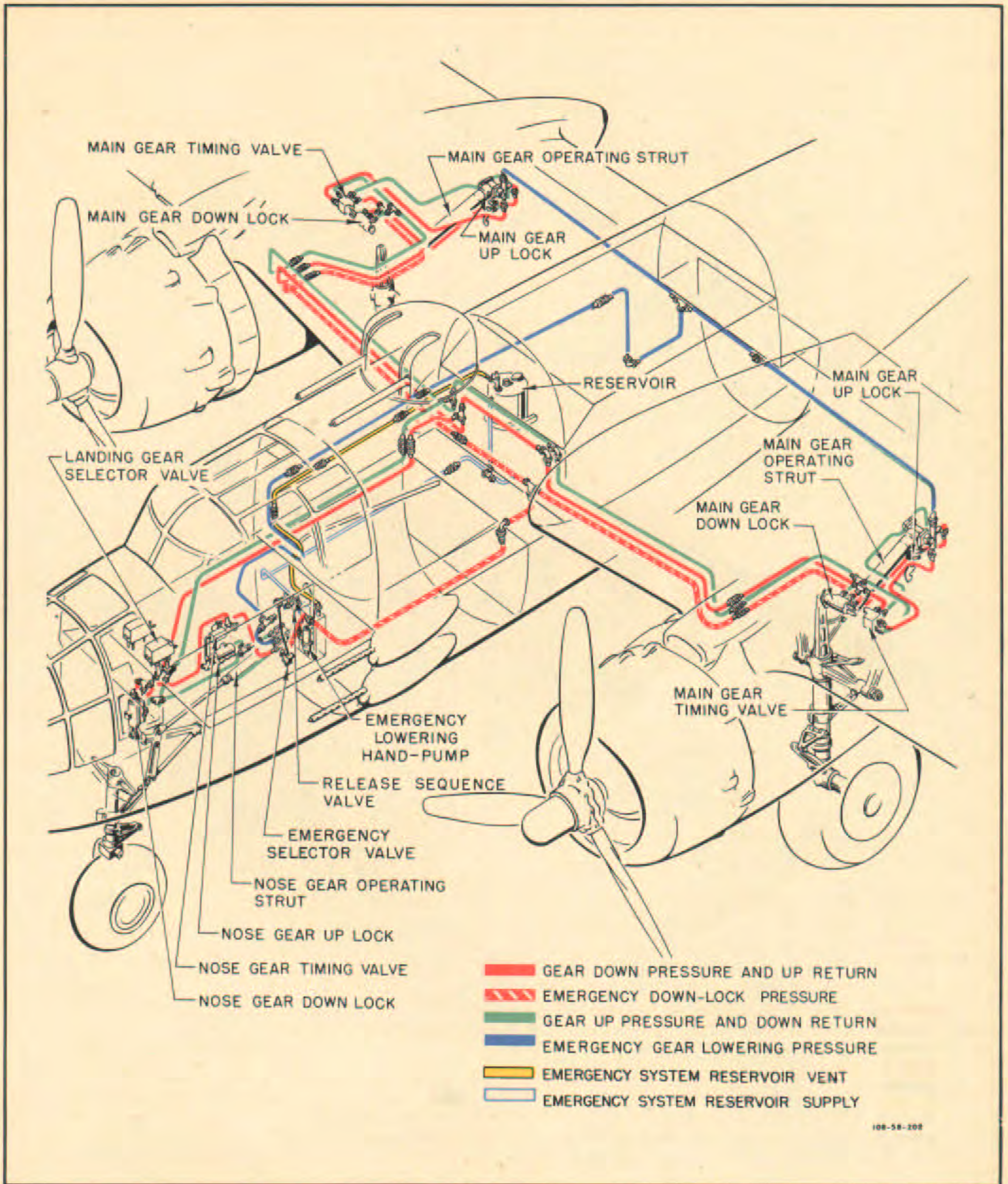
Figure 8—Hydraulic Landing Gear System
