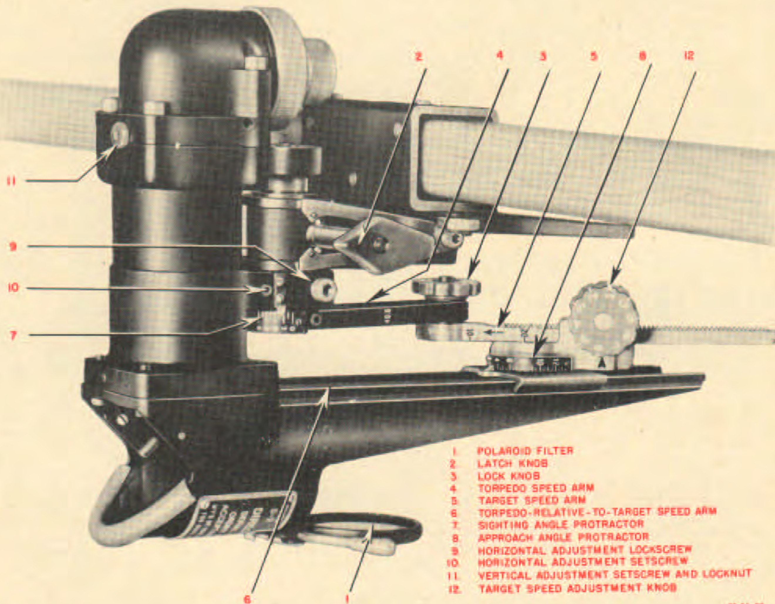
Figure 38—Torpedo Director
