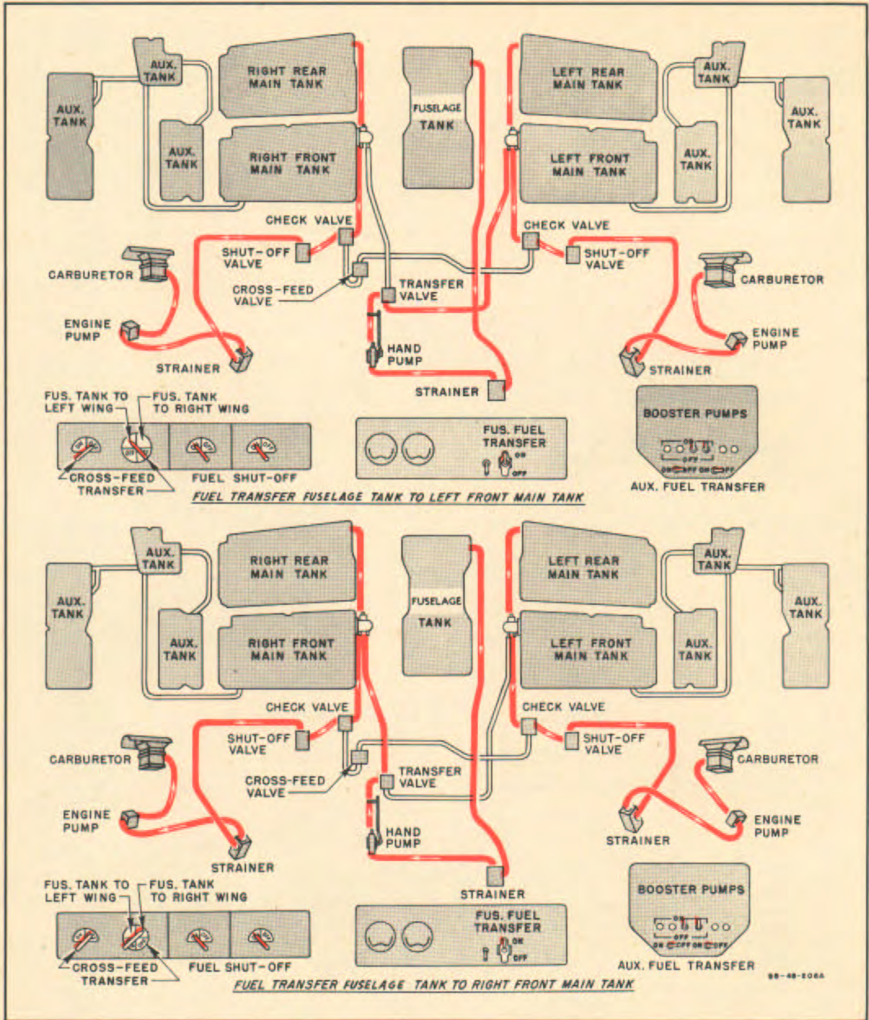
Figure 23—Fuel System Management—Fuel Transfer
