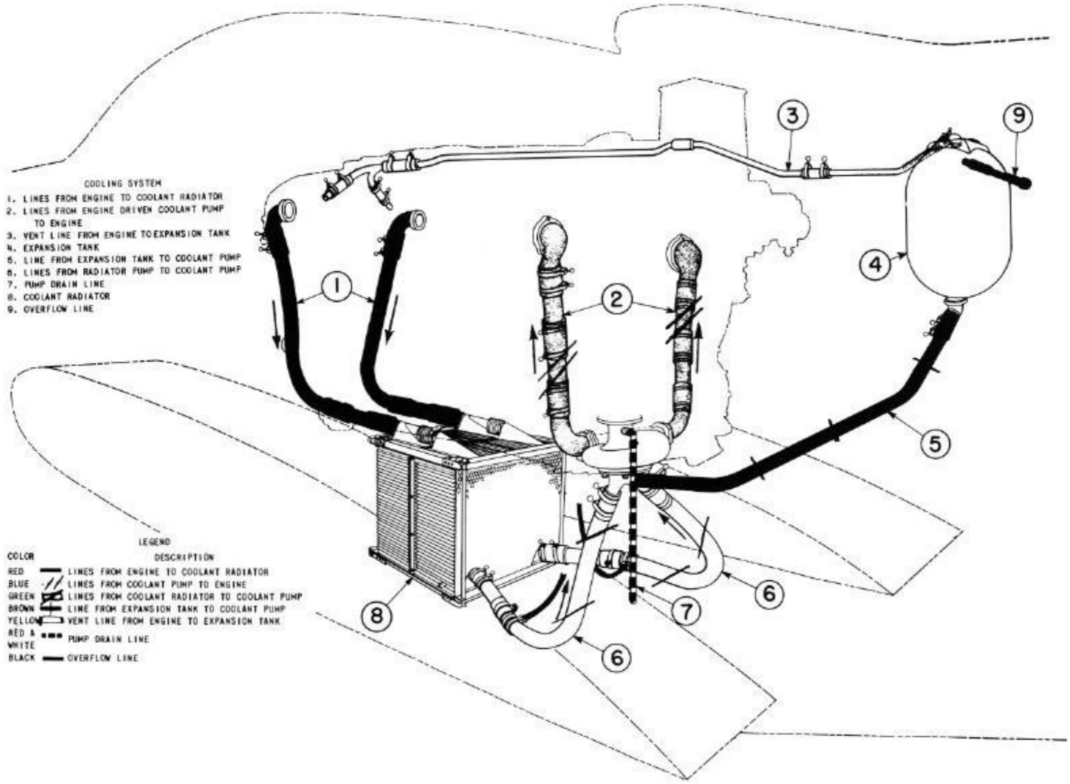
Figure 11 - Cooling System
