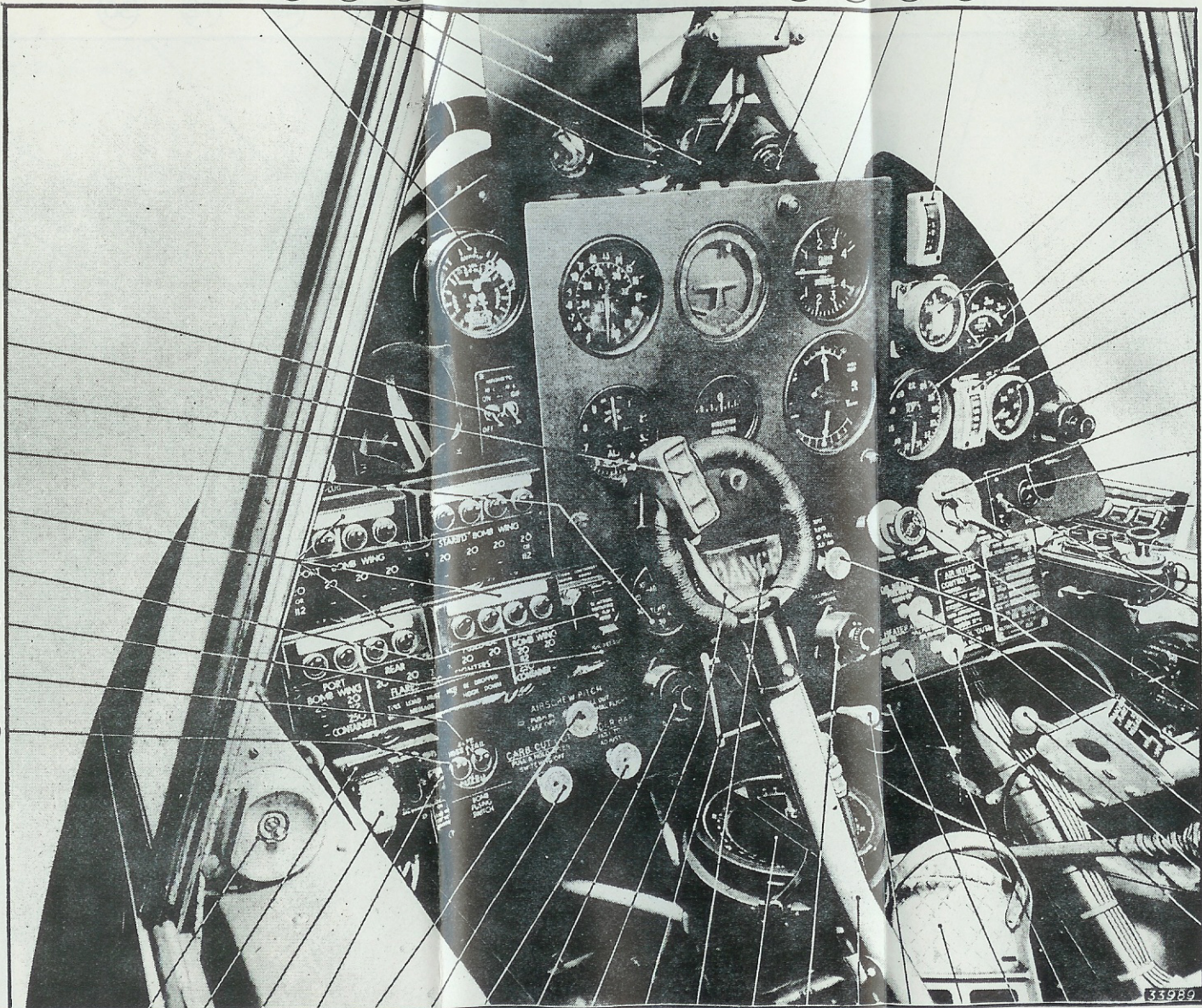
PILOT'S INSTRUMENT PANEL - VIEW TO STARBOARD
