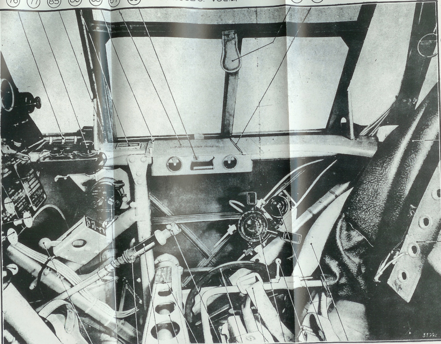
STARBOARD SIDE OF PILOT'S COCKPIT
